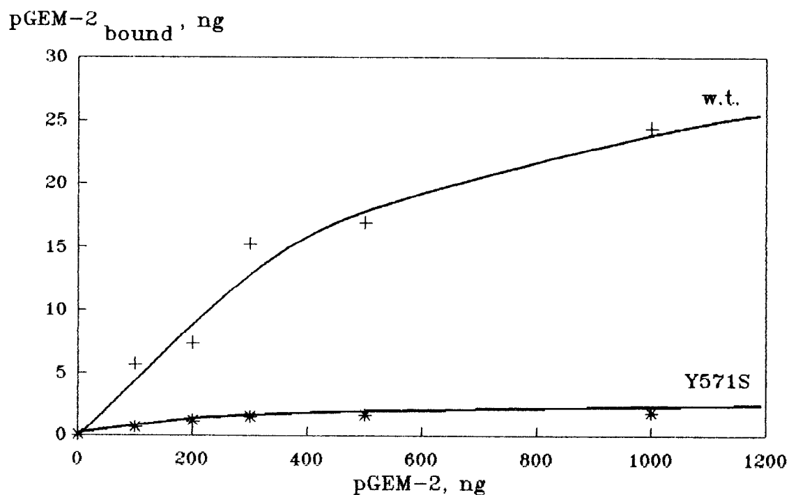
Fig. 5. Binding of the w.t. T7 RNAP and the Y571S mutant to the ^{32}\text{P} -end-labeled pGEM-2 linearized with EcoRI .
